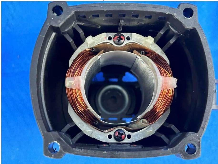
Photo 17 Description: Stator
