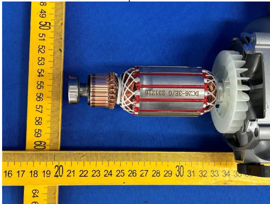
Photo 19 Description: Rotor
